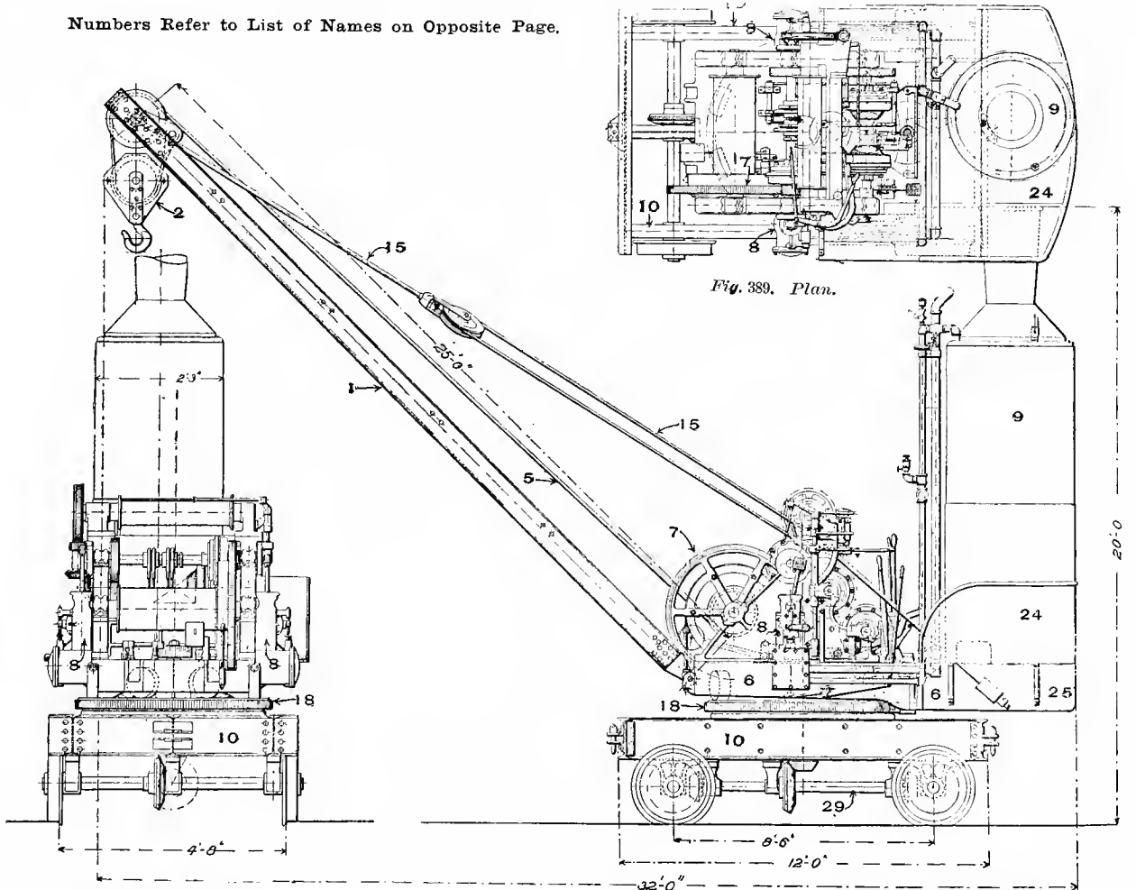
Fig. 391. Side Elevation.
